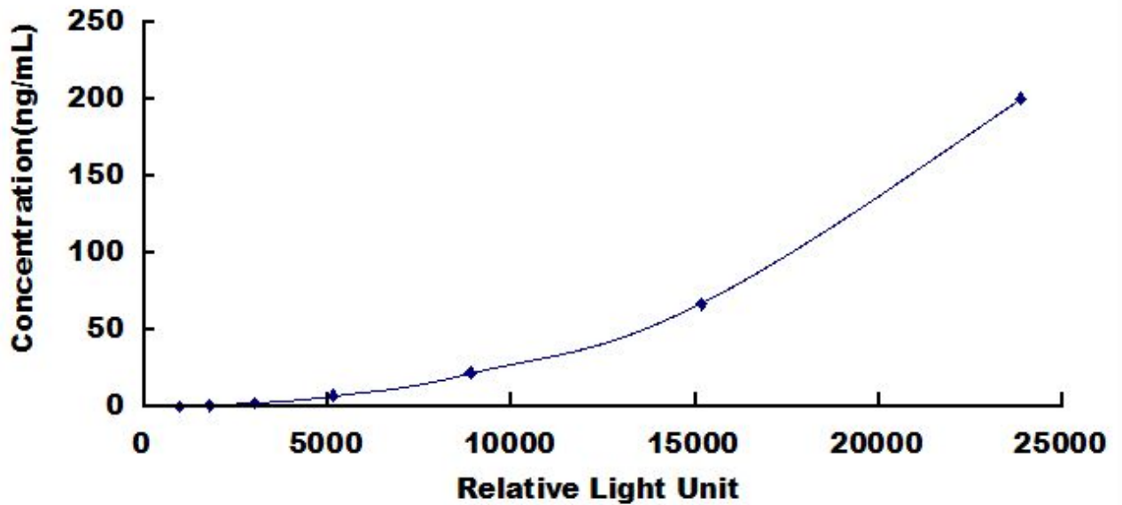
Typical Standard Curve for C5a, Rat CLIA.
